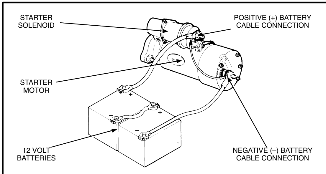
Figure 4–14. Typical Electric Starter Motor Connections (24 Volt System Shown)
