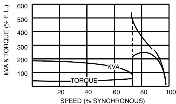
TYPICAL TORQUE AND KVA CURVES FOR SQUIRREL CAGE INDUCTION MOTORS
