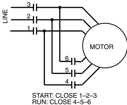
MOTOR STARTING DIAGRAM
