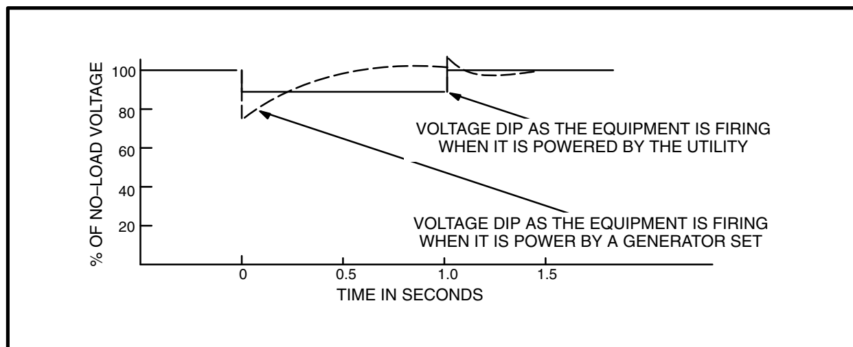
Figure 3-1. Voltage Dip in Medical Imaging Applications
