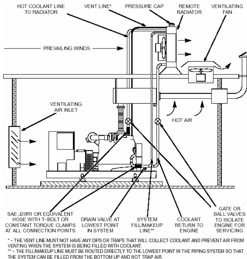
Figure 6–24. Typical Remote Radiator System
