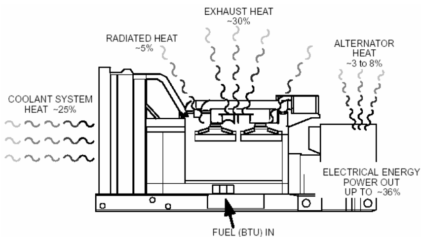
Figure 6–14. Typical Generator Set Heat Balance
