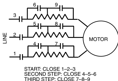
MOTOR STARTING DIAGRAM
