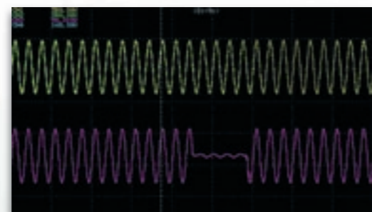
Utility and generator synchronized voltage Load voltage
